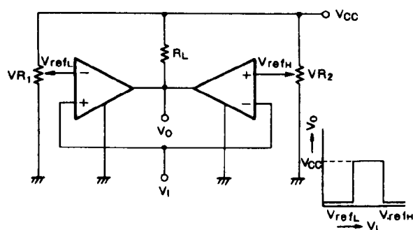
(9) Window comparator
