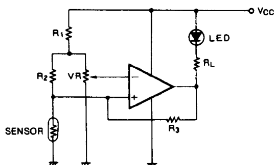
(7) Sensor detector
