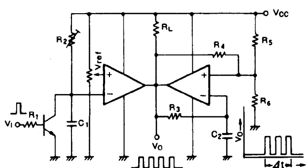
(10) Pulse train generator
